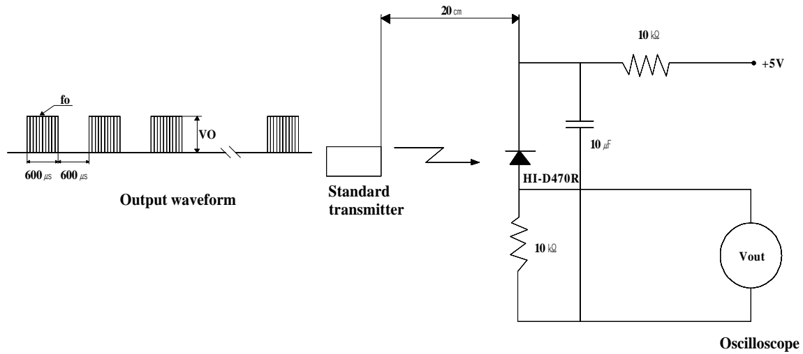
Fig.1 Standard transmitter
