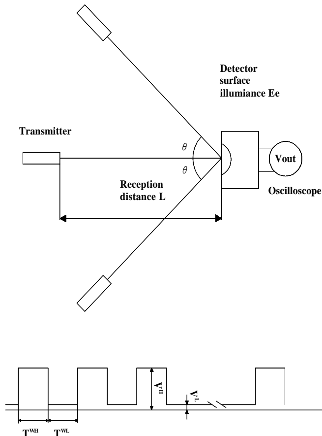
Fig.2 Standard optical test system
